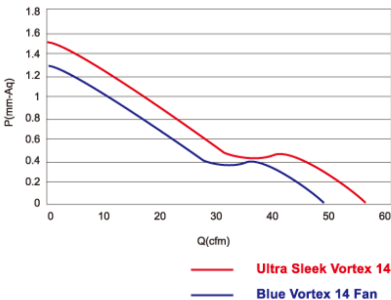
P-Q Curve
